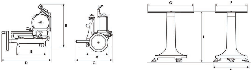
Measurements: A:13.4" B: 15.7" C: 23.6" D:28.3" E:29.1" F:28" H: 27.5" I:33.5"
